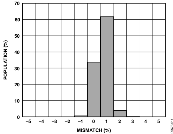
Figure 11. Self-Test Mismatch at 25°C ( V_{RATIO} = 5 V )
