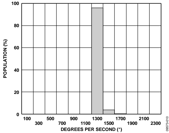
Figure 10. ST2 Output Change at 25°C ( V_{RATIO} = 5 V )
